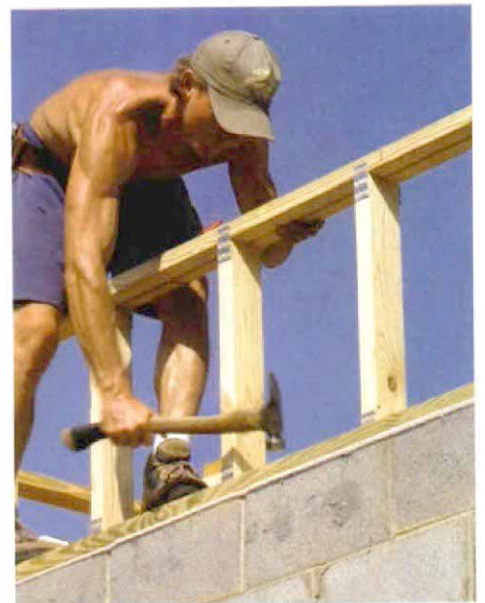
Ladder trusses go along outside walls. Ladder trusses are made specifically for outside walls, where their vertical webs make an easier target for sheathing and siding nails than diagonal webs would be.
